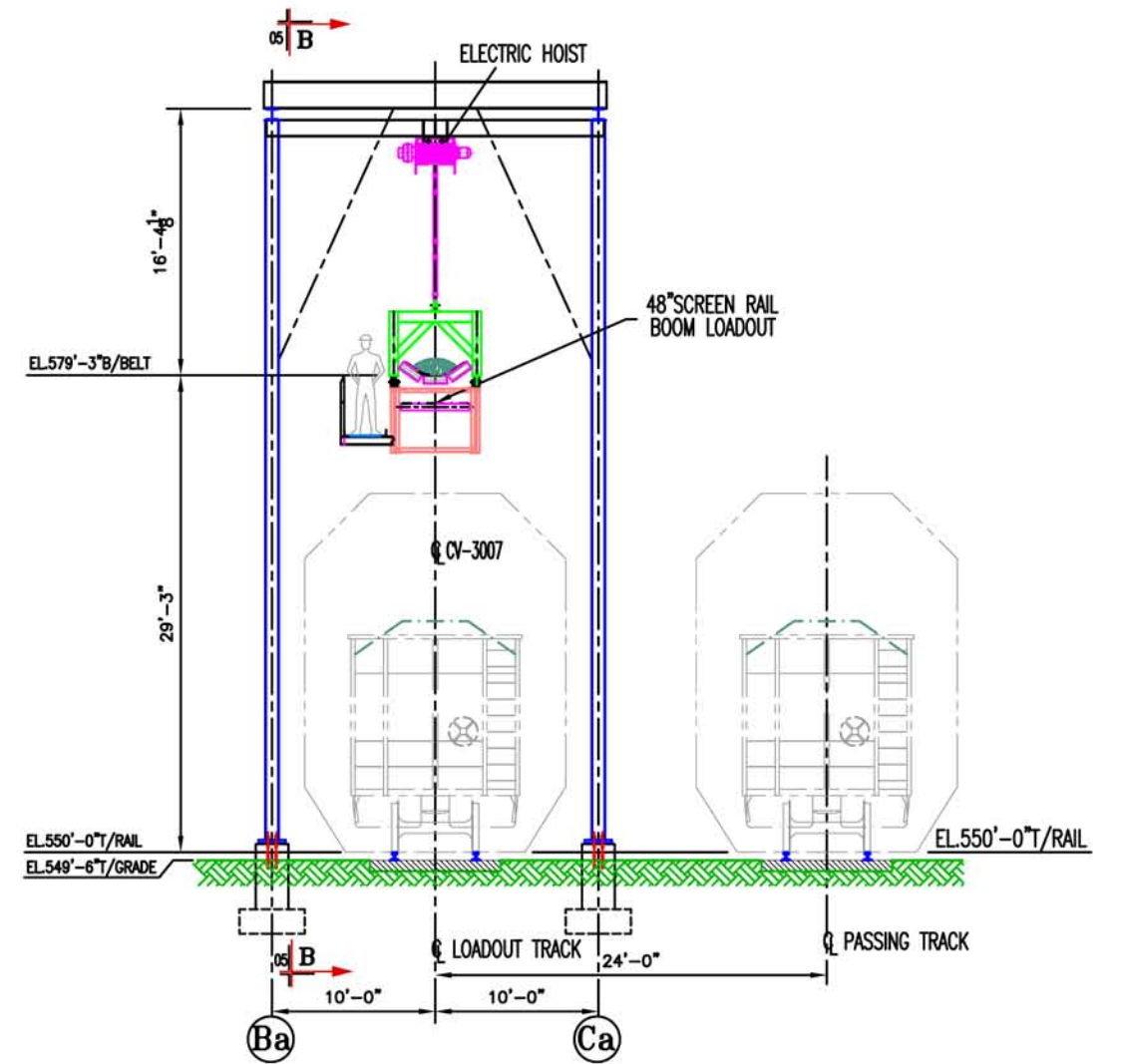
SECTION E-E
